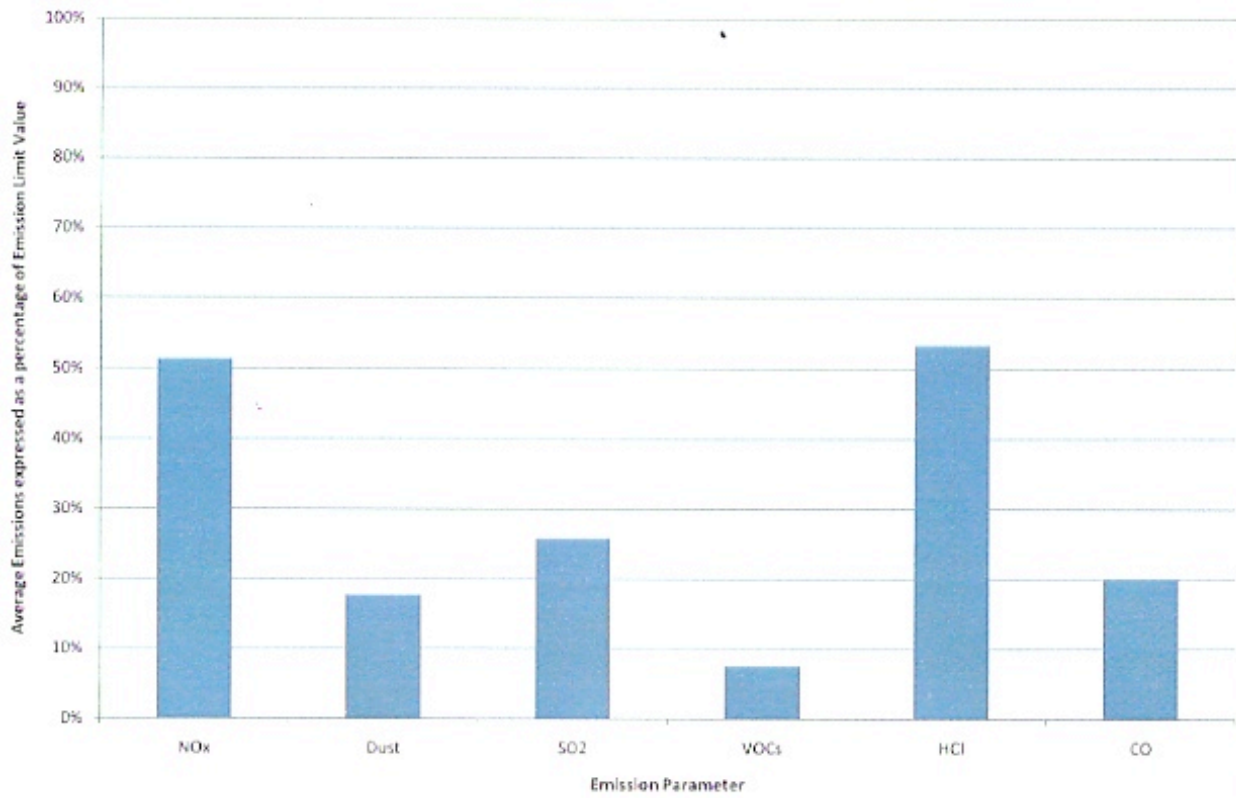
Unit 1 Emissions March 2011
