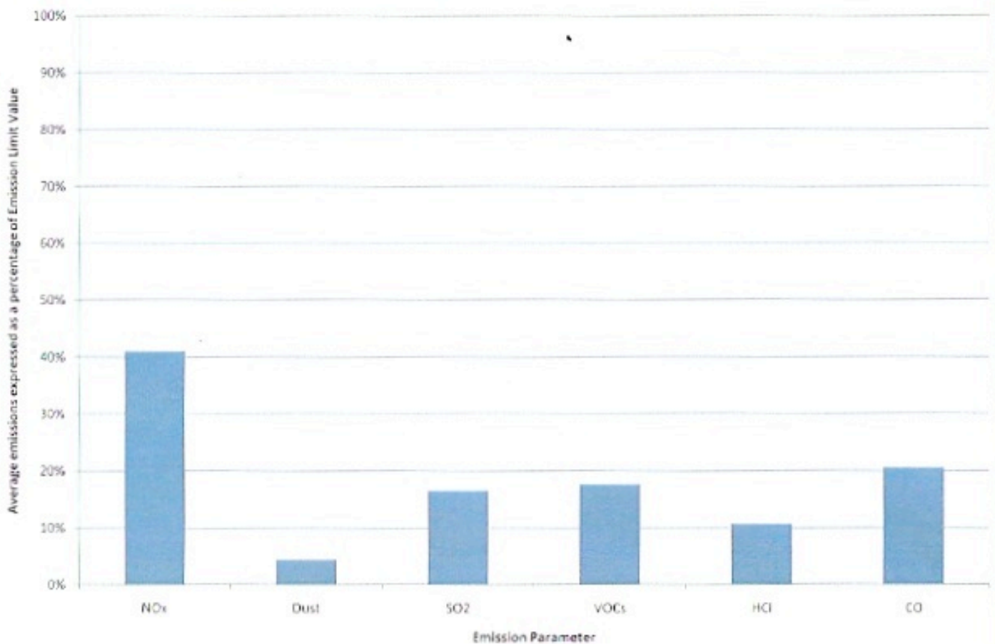
Unit 2 Emissions January 2011
